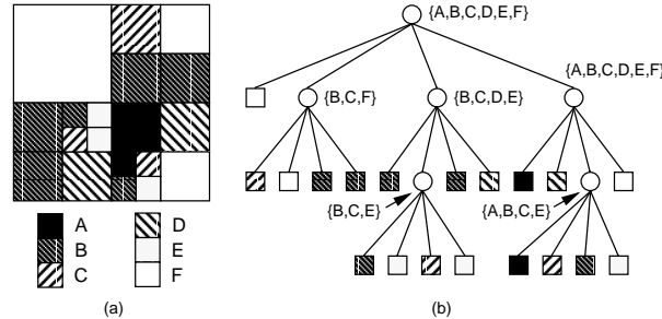
Figure 5: (a) Sample non-binary image, and (b) its corresponding truncated pyramid.
